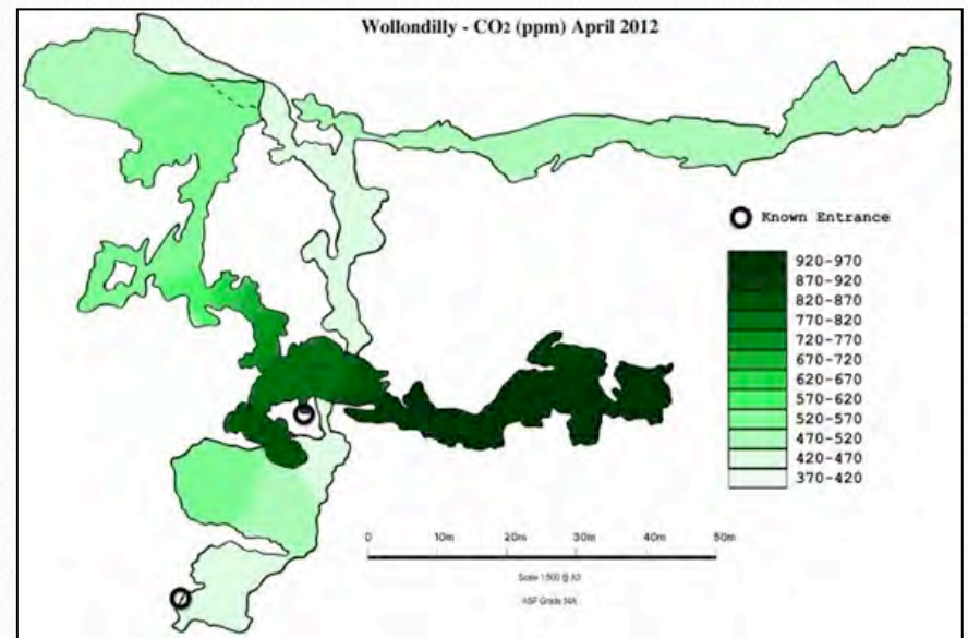
FIGURE 1 a. Cave carbon dioxide (CO 2 ppm) distribution map for Wollondilly cave, April 2012.
