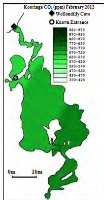
FIGURE 2 a. Cave carbon dioxide ( \text{CO}_2 ppm) distribution map for Kooringa cave, February 2012.
