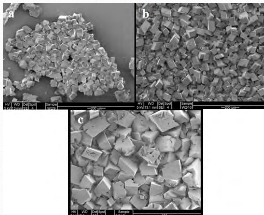
FIGURES 5 a-c. SEM Images of Calcite samples collected from site W2 between 2009 and 2012.
