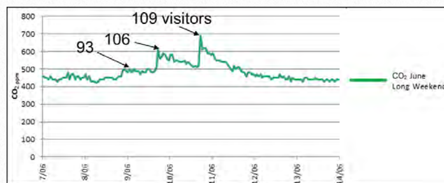
FIGURE 3. Anthropogenic impacts on \text{pCO}_{2\text{cave}} due to increased tourist activity over the June long weekend, 2012. \text{CO}_2 values returned to baseline values within 36 hours.
