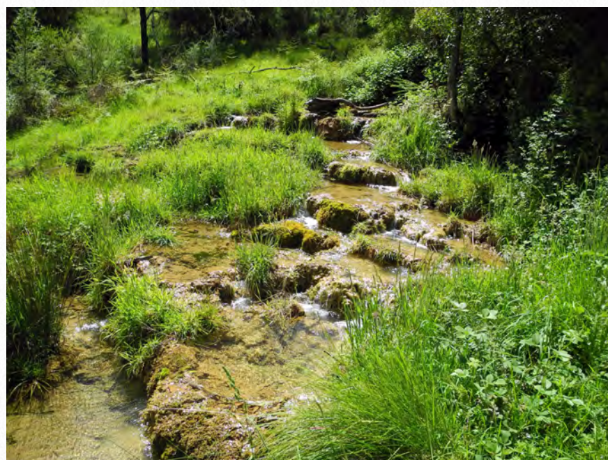
Figure 3. Scrubby Creek tufa terraces
