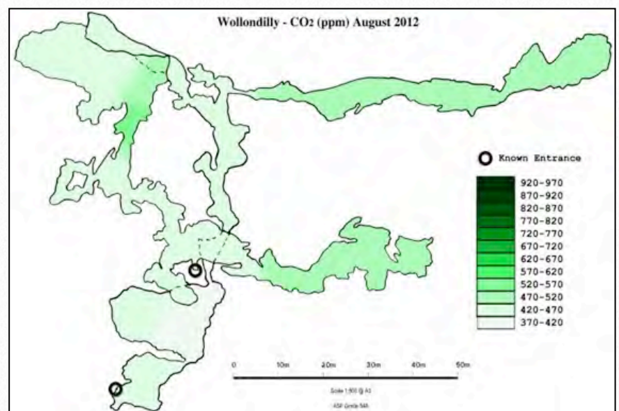
FIGURE 1 c. Cave carbon dioxide (CO 2 ppm) distribution map for Wollondilly cave, August 2012.
