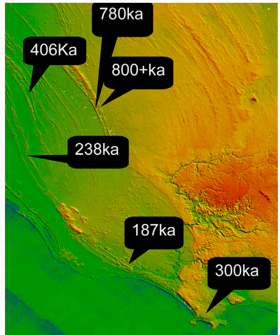
FIGURE 3. Dated dunes. Dunes dates do not include confidence levels. Dates are thermoluminescence dates from a number of published sources (Belperio, 1995 & White, 2000)
