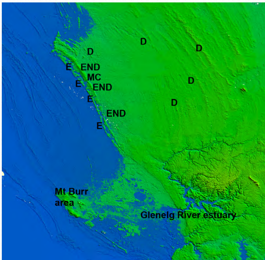
FIGURE 6. Relative Sealevel at 70 higher ASL than present showing the coastal and estuarine conditions of the Naracoorte area.
