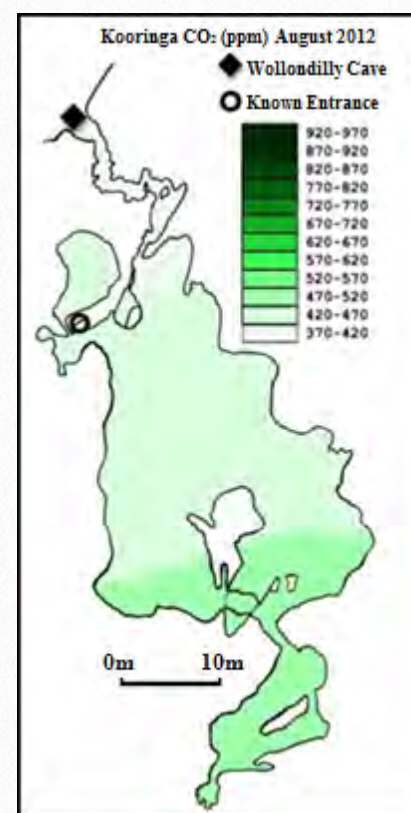
FIGURE 2 c. Cave carbon dioxide ( \text{CO}_2 ppm) distribution map for Kooringa cave, August 2012.
