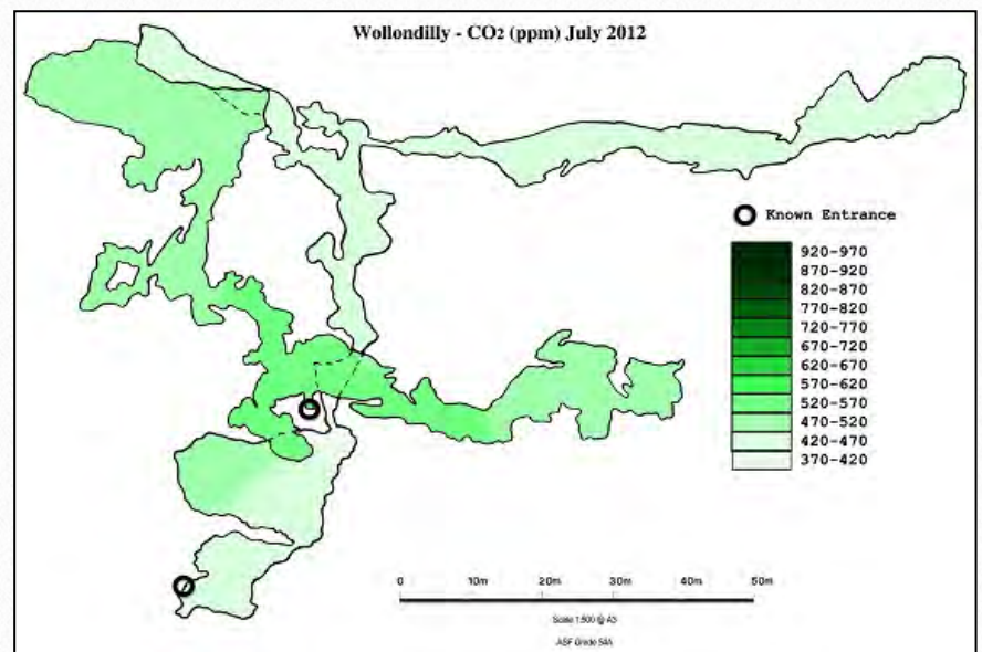
FIGURE 1 b. Cave carbon dioxide (CO 2 ppm) distribution map for Wollondilly cave, July 2012
