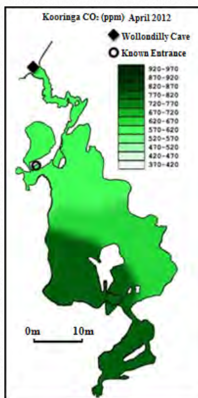
FIGURE 2 b. Cave carbon dioxide ( \text{CO}_2 ppm) distribution map for Kooringa cave, April 2012.
