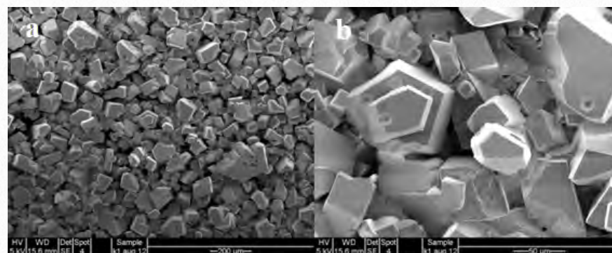
FIGURES 7 a-b. SEM Images of Calcite samples collected from site K1.
