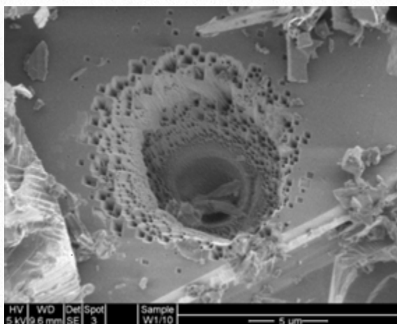
FIGURE 4 e. SEM Image of the unusual surface features of Wombeyan calcite.
