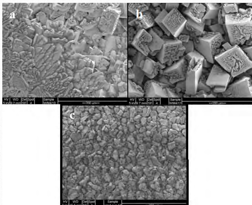
FIGURES 6 a-c. SEM Images of Calcite samples collected from site WM4 between 2009 and 2012.
