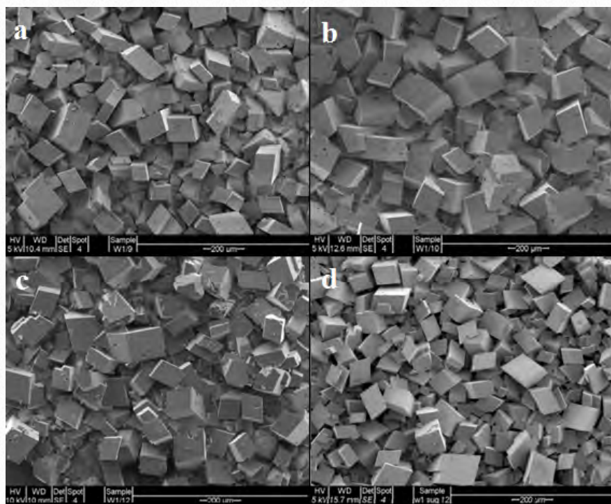
FIGURES 4 a-d. SEM Images of Calcite samples collected from site W1 between 2009 and 2012.
